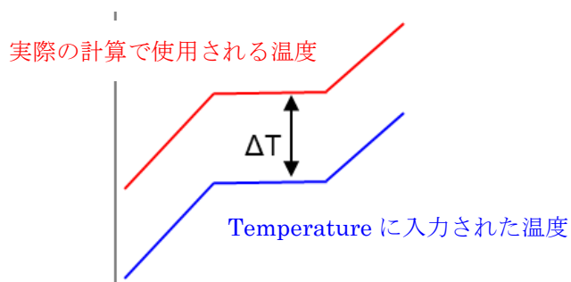
(例 2) Piecewise Linear
