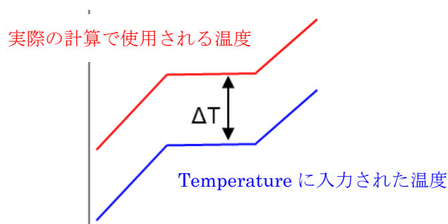
(例 2) Piecewise Linear
